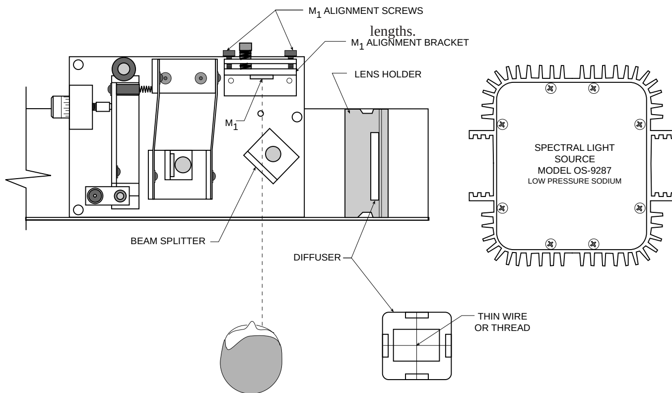
FIGURE 10 USING A SPECTRAL LIGHT SOURCE
