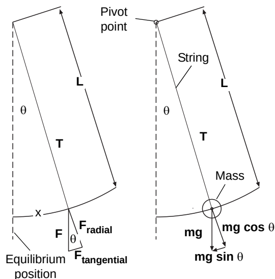
Figure 10.1: Pendulum
