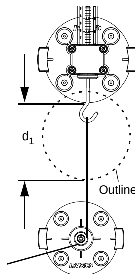
Fig. 13.3: Measure d_1
