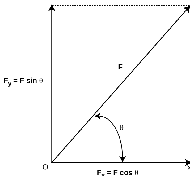
Figure 3.2: Vector components
