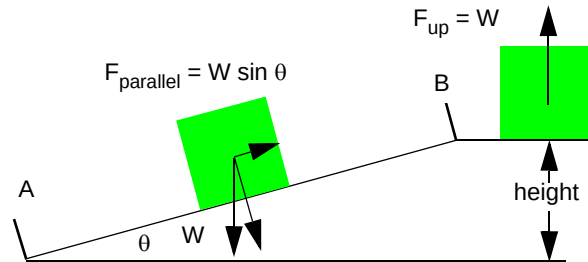
Figure 13.1: Inclined Plane
