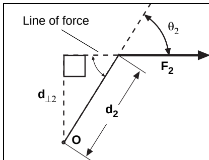
Figure 6.4: Non-Parallel Forces
