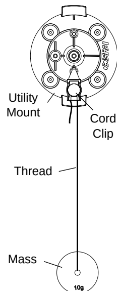
Fig. 10.2: Setup
