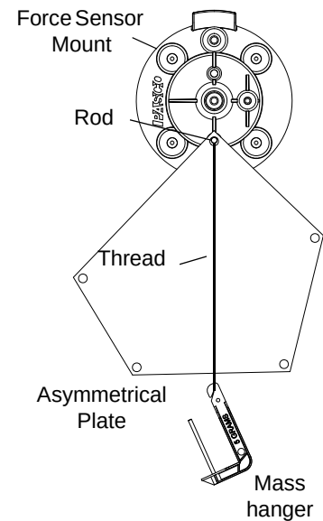
Figure 5.3: Finding the Center of Mass
