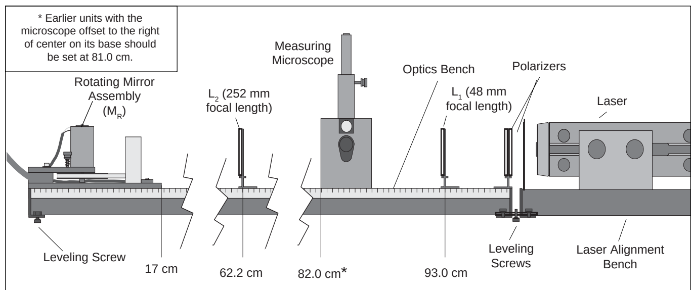
Figure 5: Equipment Alignment
