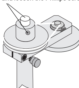
Figure 6: Adjusting the height of the pendulum bob
