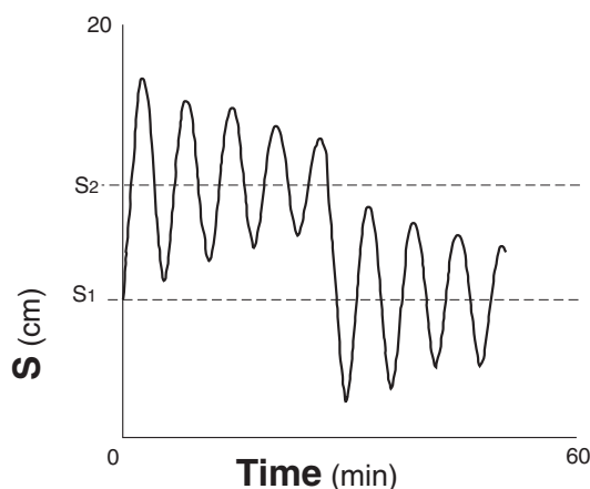
Figure 18: Typical pendulum oscillation pattern showing equilibrium positions.
