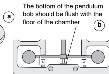
Figure 6: Adjusting the height of the pendulum bob
